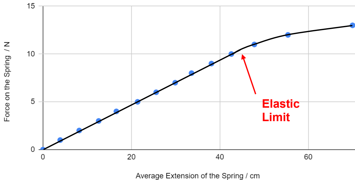
Force on the Spring / N vs Average Extension of the Spring / cm
